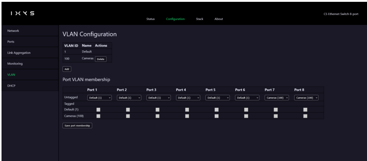
Figure 9 VLAN configuration
