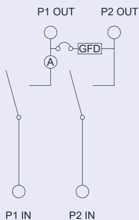
TYPICAL RELAY FUNCTION
