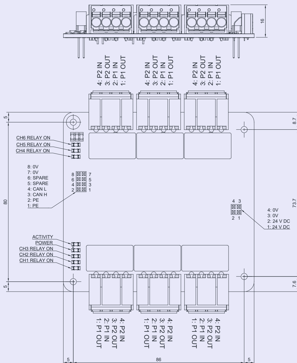
TYPICAL RELAY FUNCTION
